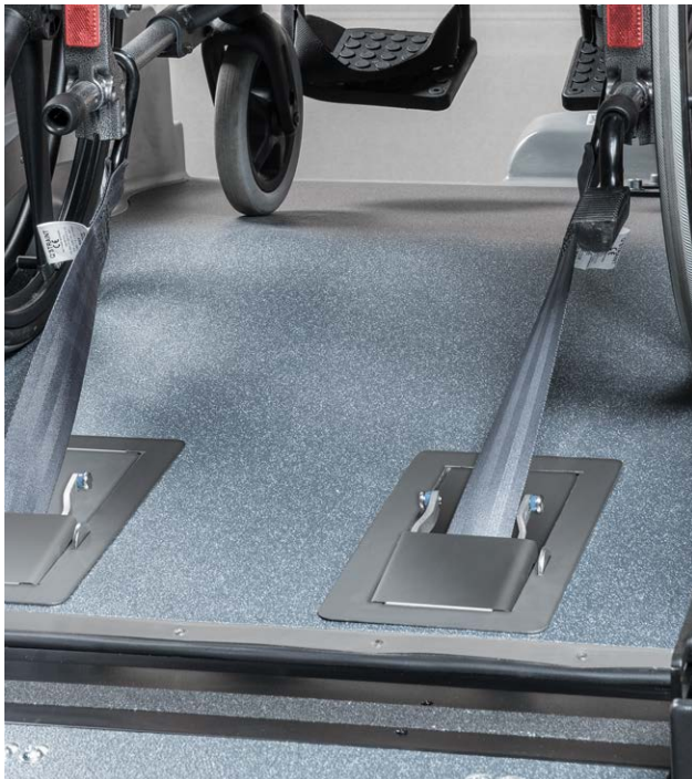
The unique patented rear impact protection system significantly increases the safety of the vehicle occupants.
